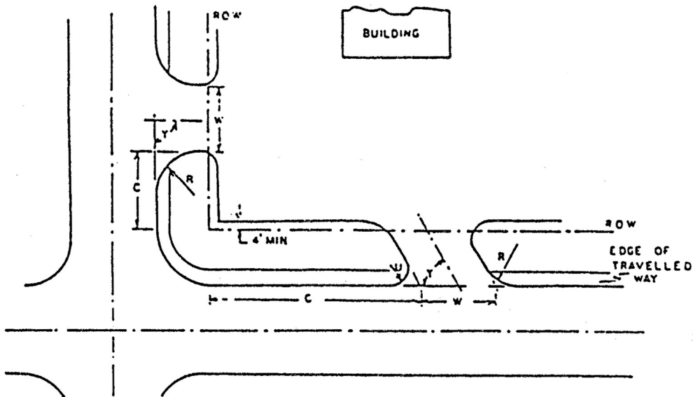
Figure 3. Driveways for Corner Installations—Diagrammatic
