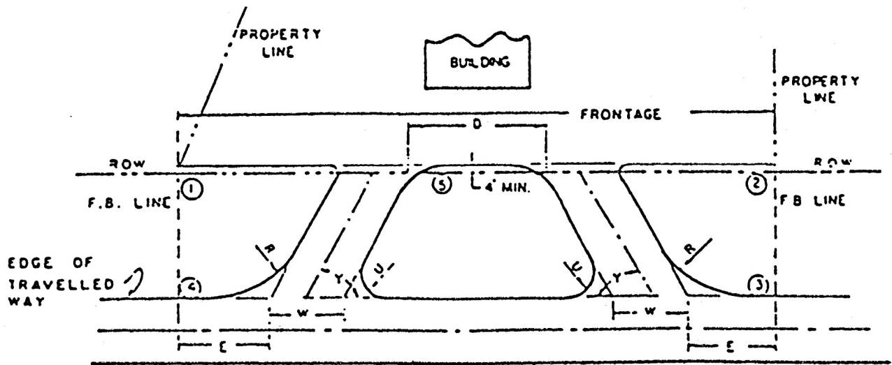
FIGURE 2. DOUBLE DRIVEWAY—DIAGRAMMATIC
