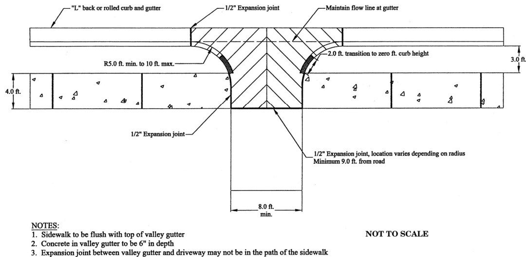
FIGURE 7. CONSTRUCTION REQUIREMENT VALLEY GUTTER, RESIDENTIAL DRIVEWAY
