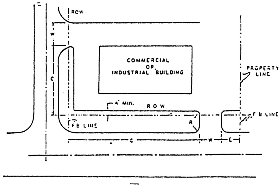
FIGURE 4. DRIVEWAYS TO A CORNER COMMERCIAL ESTABLISHMENT
