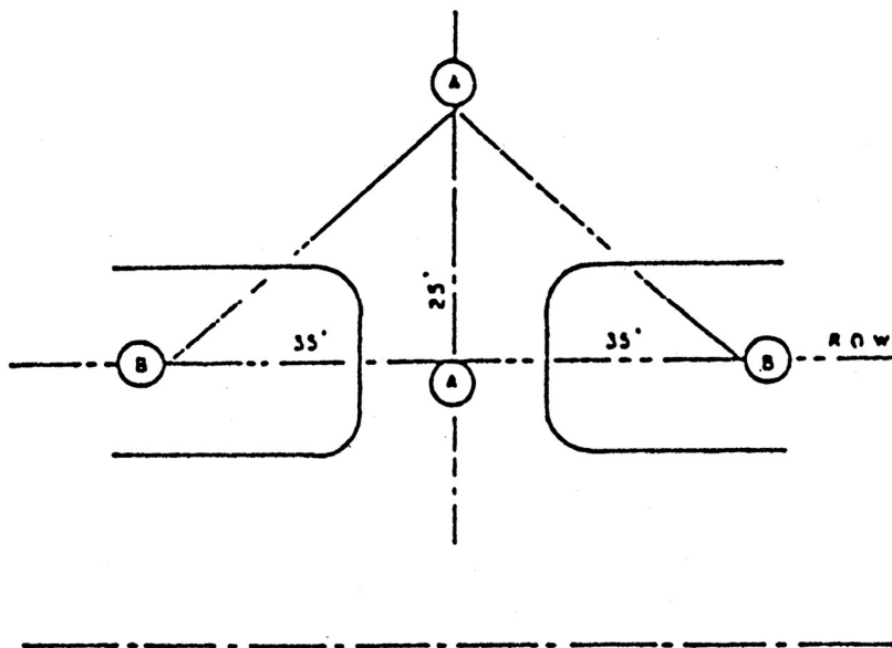
FIGURE 5A. VISIBILITY CLEARANCE (NON-RESIDENTIAL)
