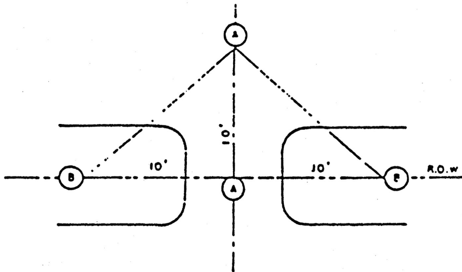
FIGURE 5B. VISIBILITY CLEARANCE (RESIDENTIAL)
