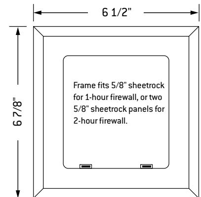
Intumescent Pad
