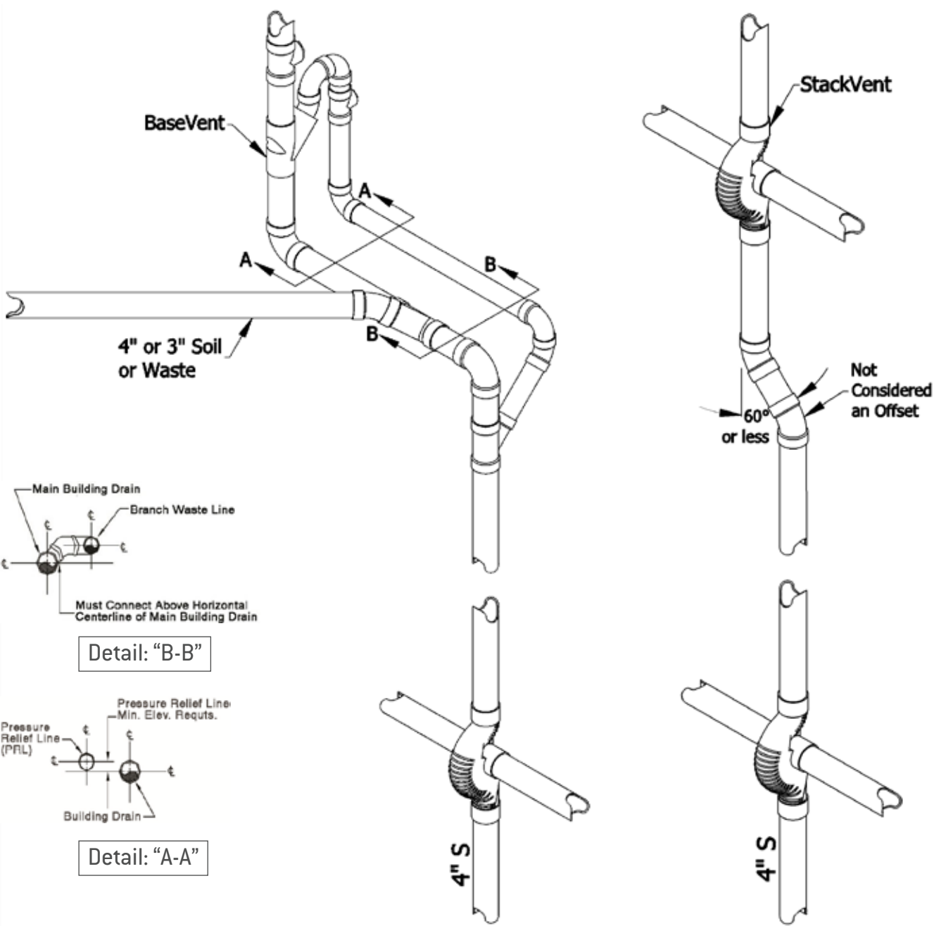
Drawing 1.5
