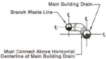
Detail: "B-B"
