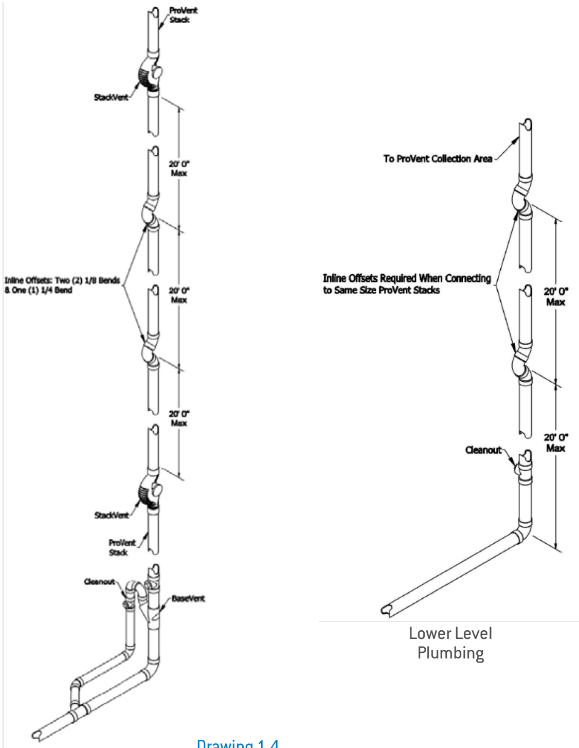
Drawing 1.4
