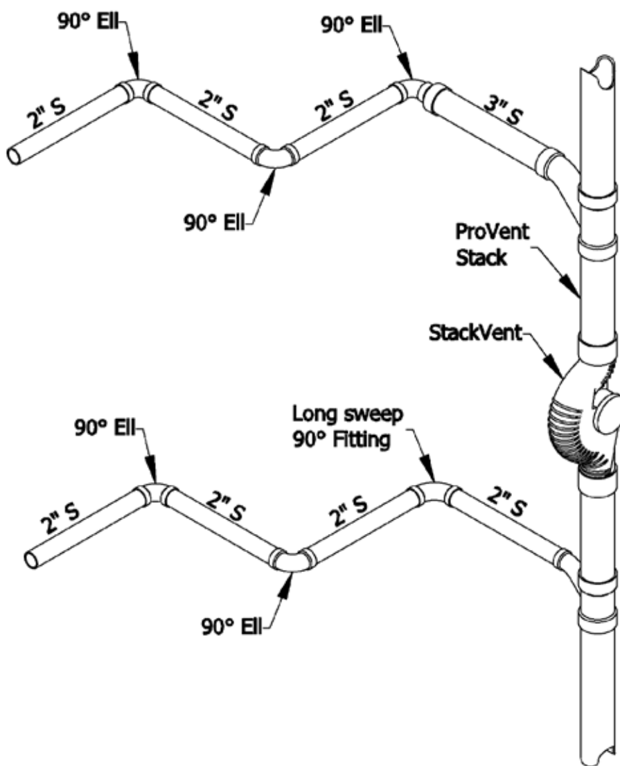
Drawing 3.2
