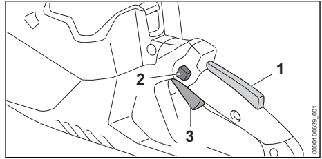
Ergo-Lever (1), Trigger Switch Lockout (2) and Trigger Switch (3)
