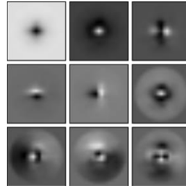
Figure 2: Convolution basis.
