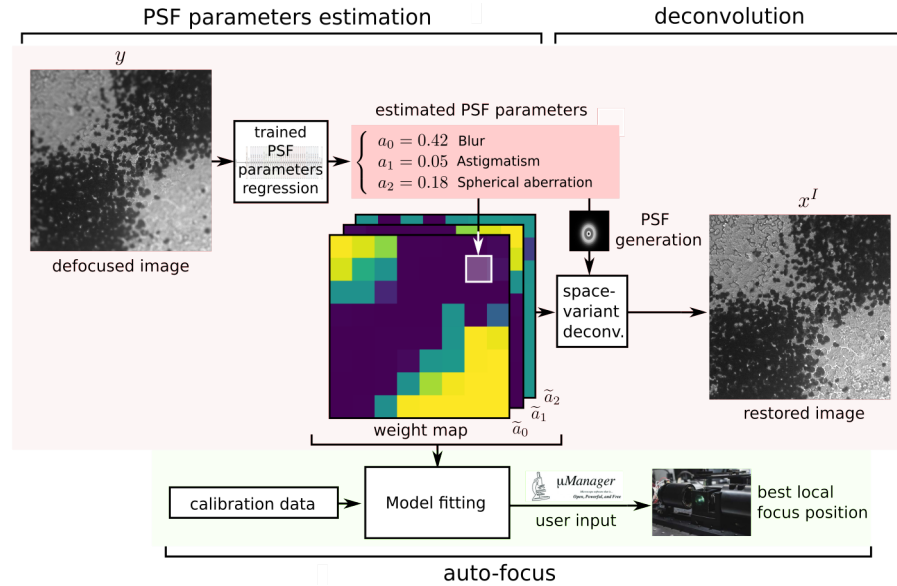
Fig. 1 Method to estimate a map of local PSFs that degraded an image that can be fed into a spatially variant deconvolution algorithm or an auto-focus algorithm.
