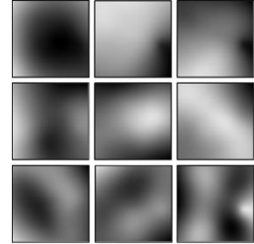
Figure 3: Coefficients basis.
