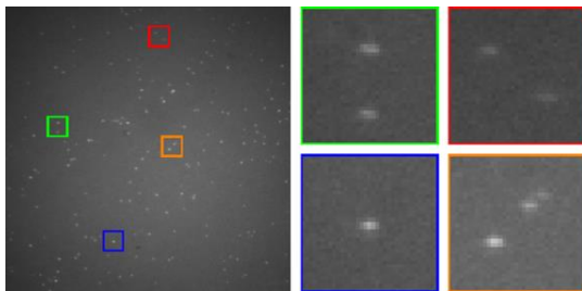
Figure 1: Sampled PSFs.
