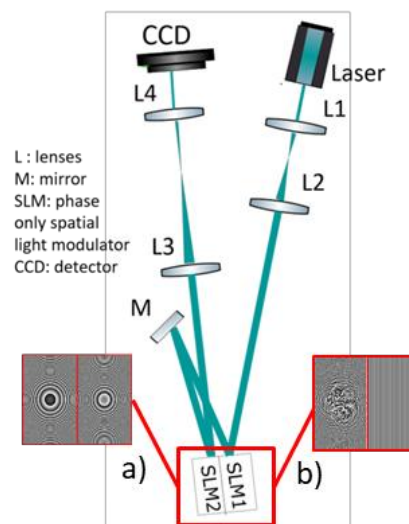
Figure 1. Illumination setup with two different modes to choose.
