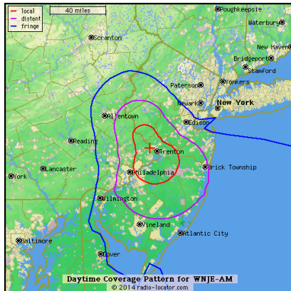
Coverage map of 920 AM The Jersey (WNJE), located in Princeton, NJ, is a sister station to 94.5 WPST. (courtesy Radio-Locator.com)
