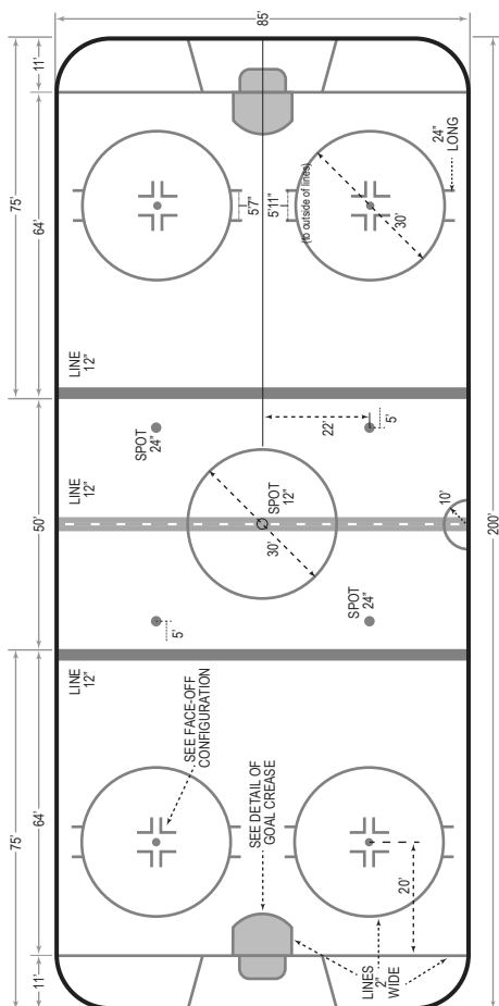
OFFICIAL DIMENSIONS OF RINK SURFACE
