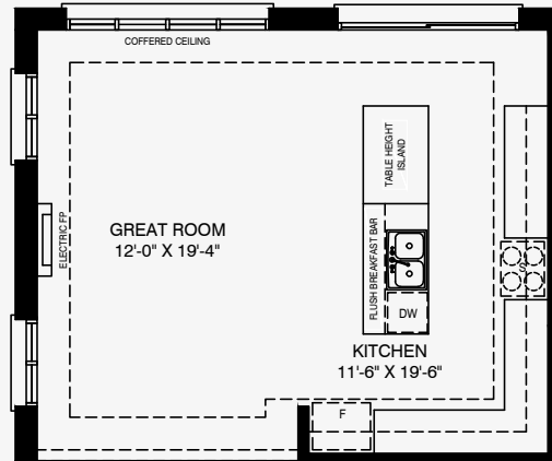
Partial Ground Floor For Opt. Modern Kitchen Elevation A
