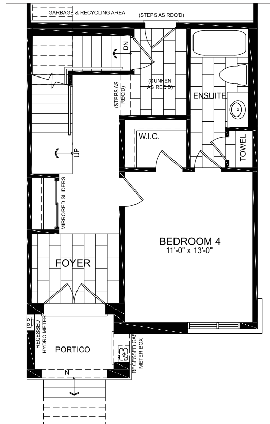
ELEVATION C1 OPT GROUND FLOOR W/ BEDROOM 4
