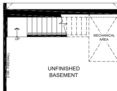
ELEVATION A1 PARTIAL BASEMENT W/O SUNKEN AREA
