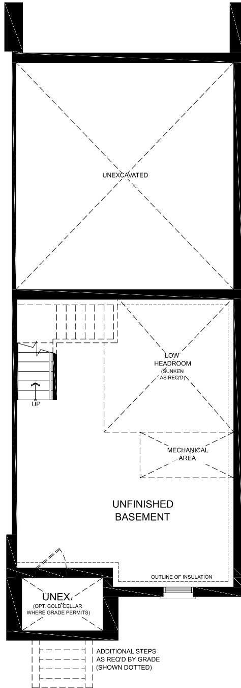
ELEVATION B1 BASEMENT
