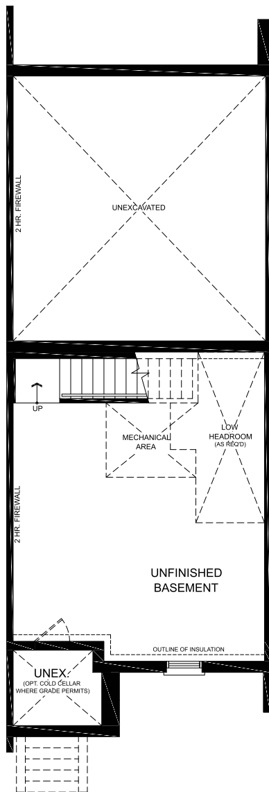
ELEVATION A1 BASEMENT
