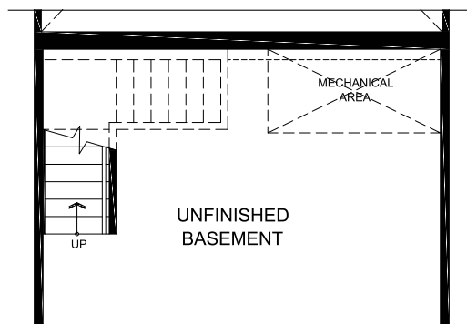
ELEVATION C1 PARTIAL BASEMENT W/O SUNKEN AREA
