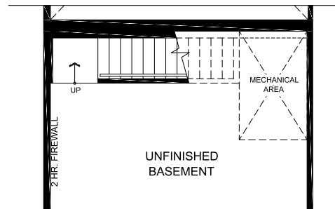
ELEVATION C1 PARTIAL BASEMENT PLAN W/O SUNKEN AREA
