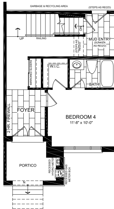
ELEVATION C1 OPT GROUND FLOOR W/ BED 4
