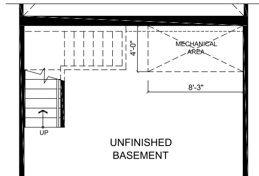
ELEVATION A1 PARTIAL BASEMENT W/O SUNKEN AREA
