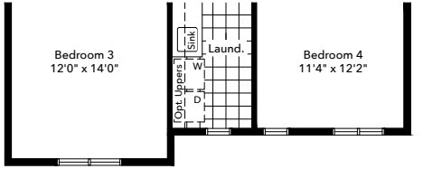
Partial Second Floor 4 Bedroom (Elevation B)
