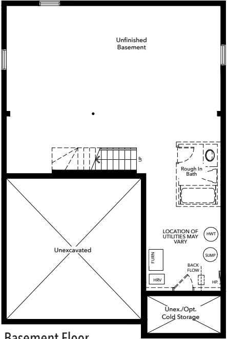
Basement Floor (Elevation A)
