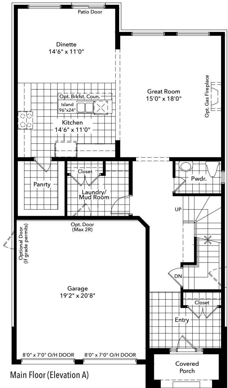
Elevation A - 2643 sq. ft.
