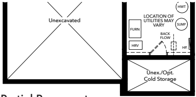
Partial Basement Floor (Elevation C)
