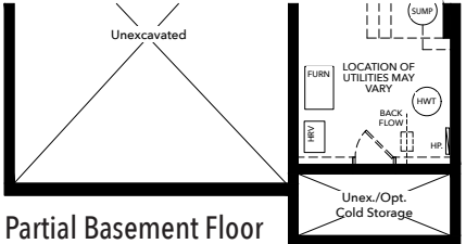
Partial Basement Floor (Elevation B)
