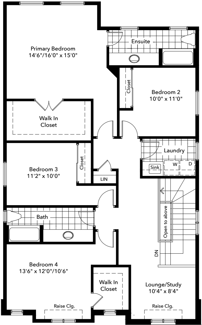
Second Floor 4 Bedroom (Elevation A)
