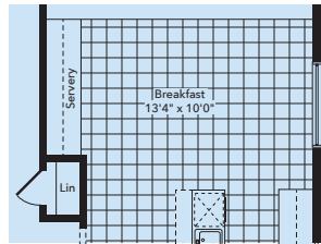
Main Floor (Optional Servery)
