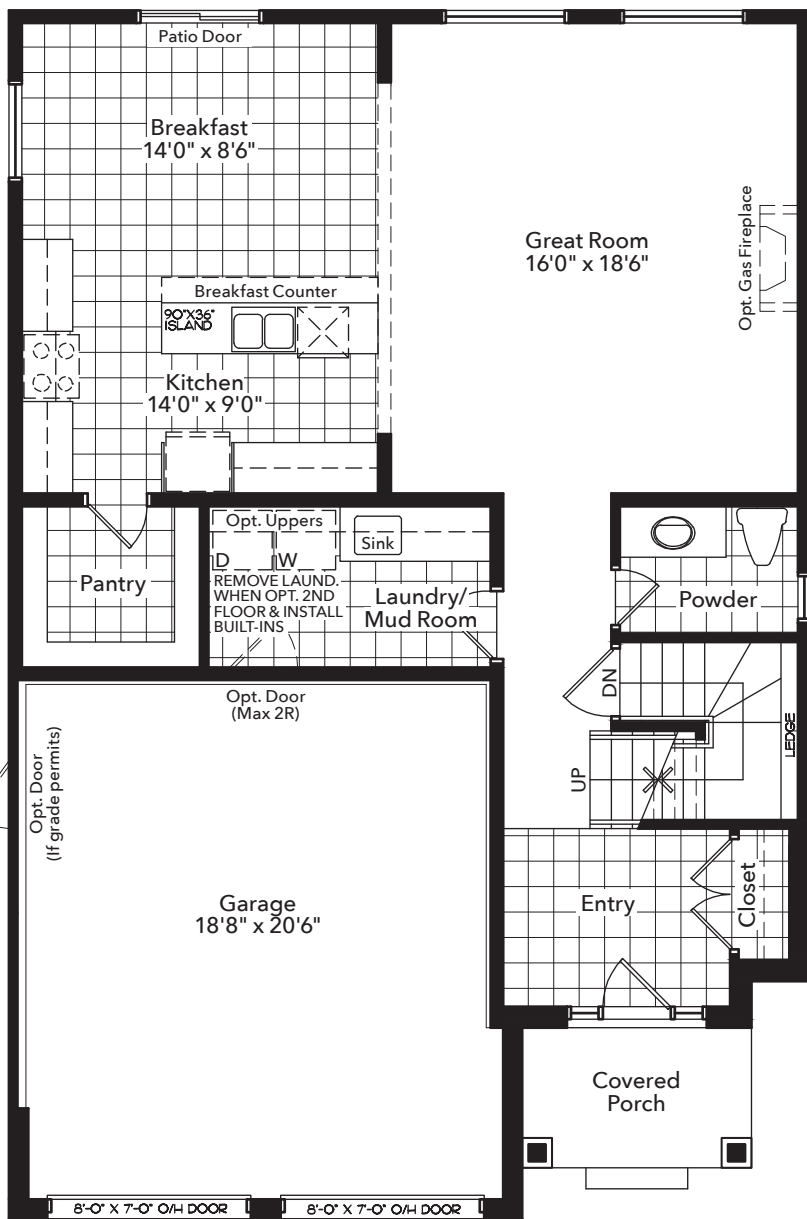
Standard Main Floor (Elevation A/B)
