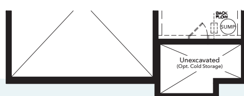
Basement Floor (Elevation B)
