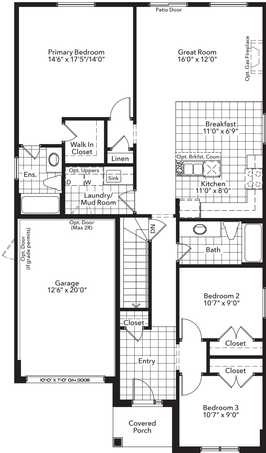
Standard Main Floor (Elevation A)
