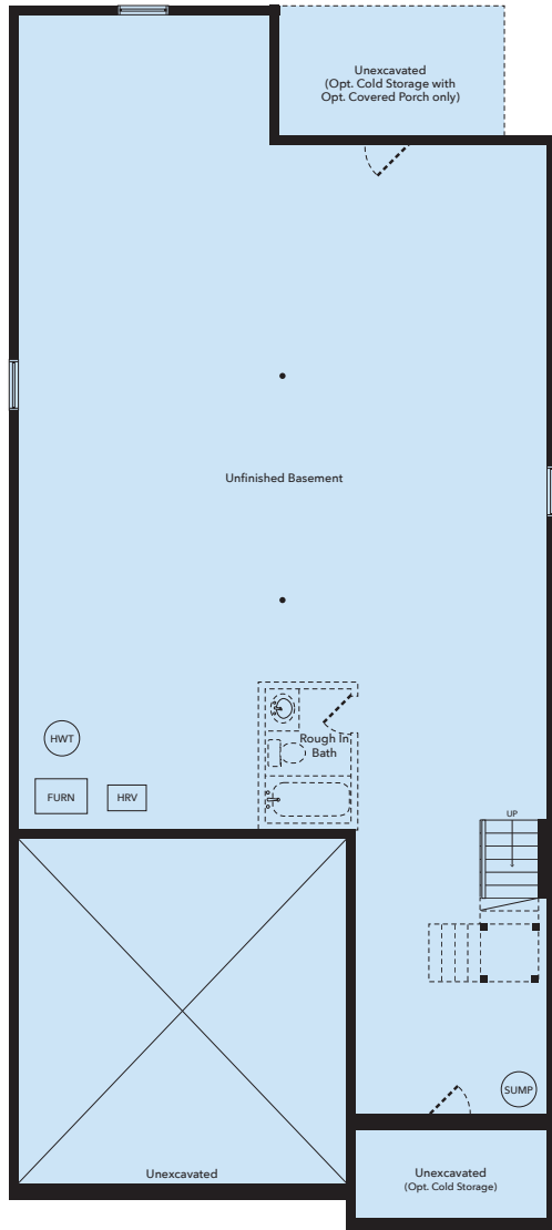
Basement A (Standard)
