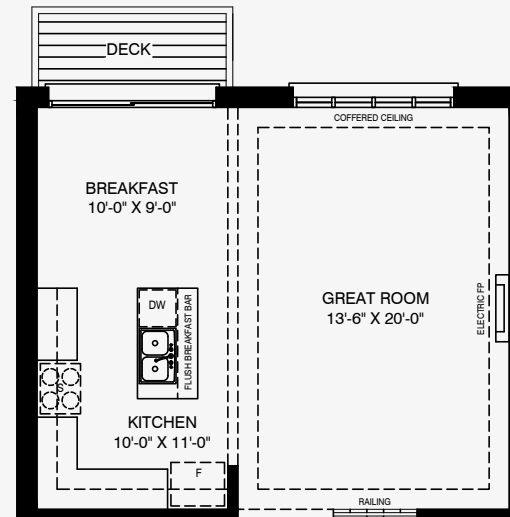
Partial Ground Floor For Walk-out Basement Elevation A2
