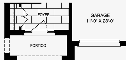
Partial Ground Floor Elevation B
