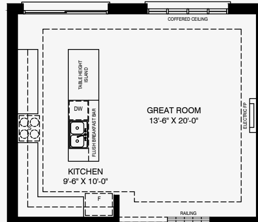
Partial Ground Floor For Opt. Modern Kitchen Elevation A1, A2
