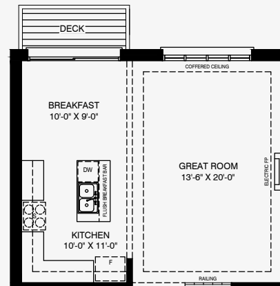
Partial Ground Floor For Walk-out Basement Elevation B
