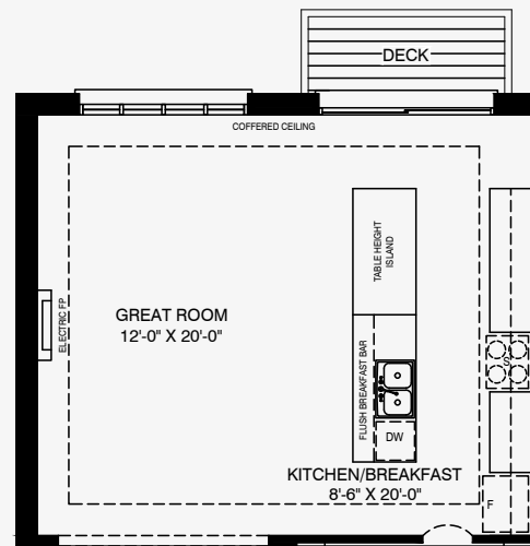
Partial Ground Floor For Opt. Modern Kitchen Elevation A
