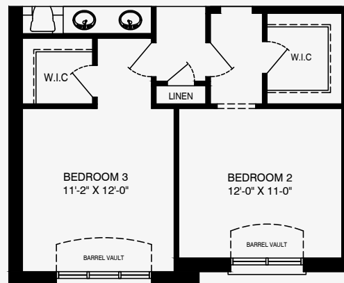
Partial Second Floor Elevation B
