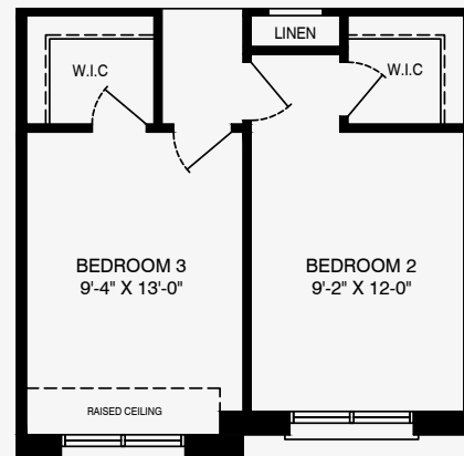
Partial Second Floor Elevation A2
